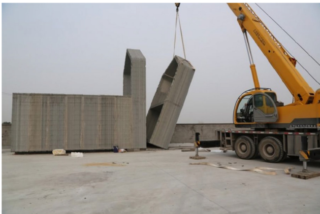
Figure 4 Assembly process of houses printed by WinSun
