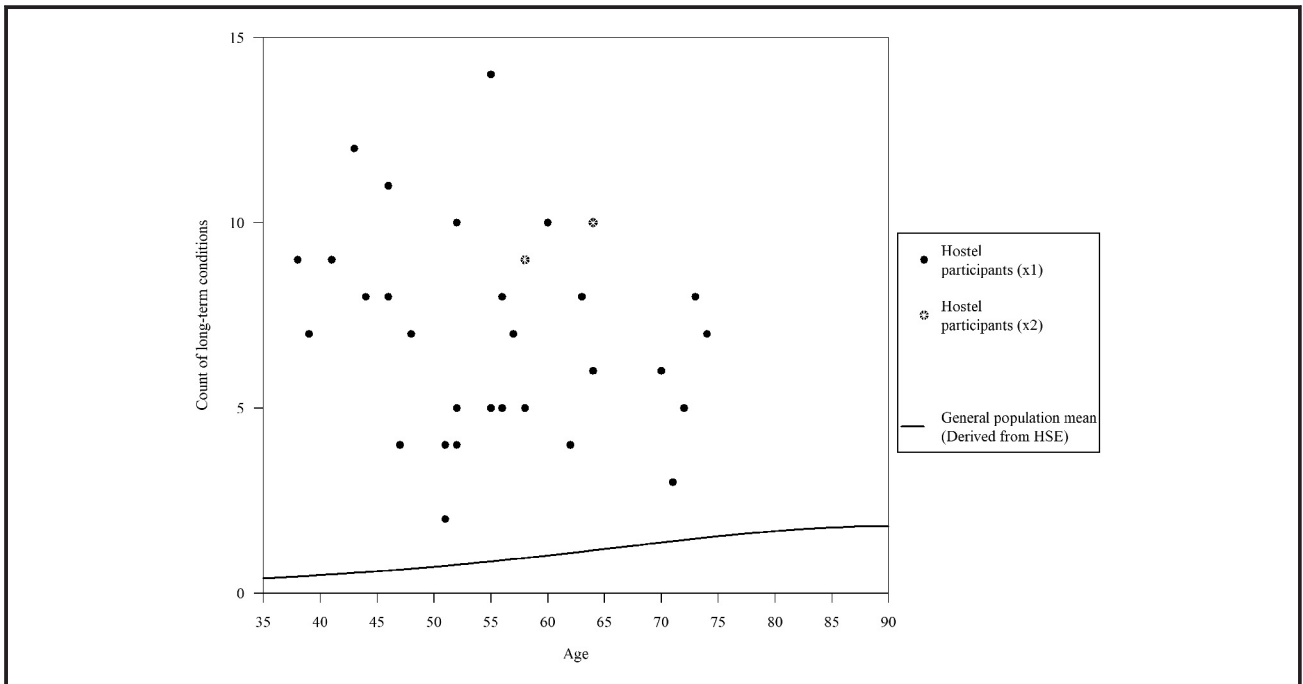
Figure 2 Multimorbidity
