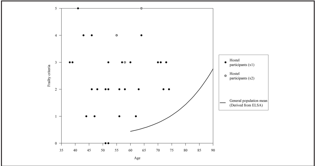
Figure 1 Frailty
